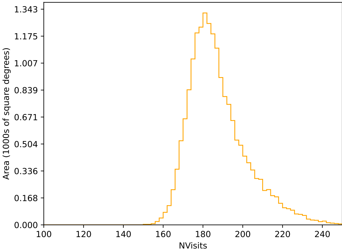
roll_pause_mjdp120_v3.4_10yrs WFD r band: NVisits
