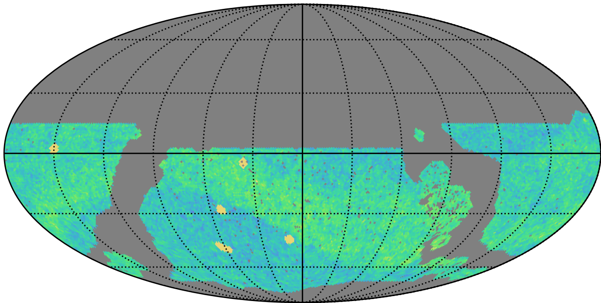
roll_pause_mjdp120_v3.4_10yrs WFD i band: NVisits
