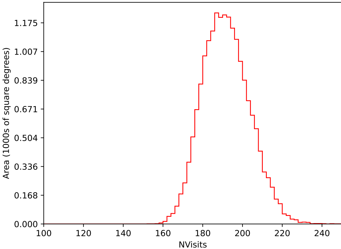
roll_pause_mjdp120_v3.4_10yrs WFD i band: NVisits
