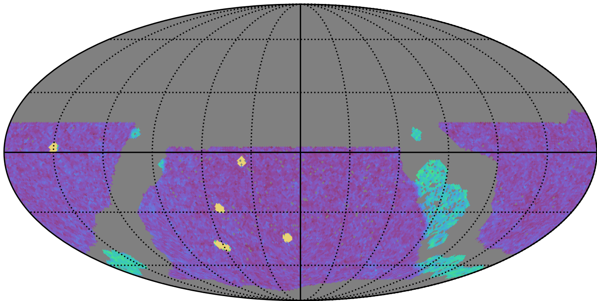
roll_pause_mjdp120_v3.4_10yrs WFD g band: NVisits
