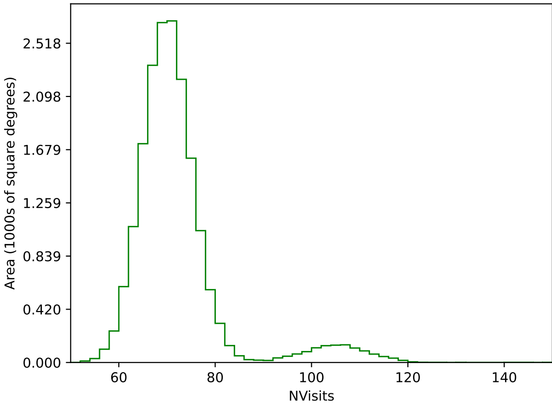
roll_pause_mjdp120_v3.4_10yrs WFD g band: NVisits
