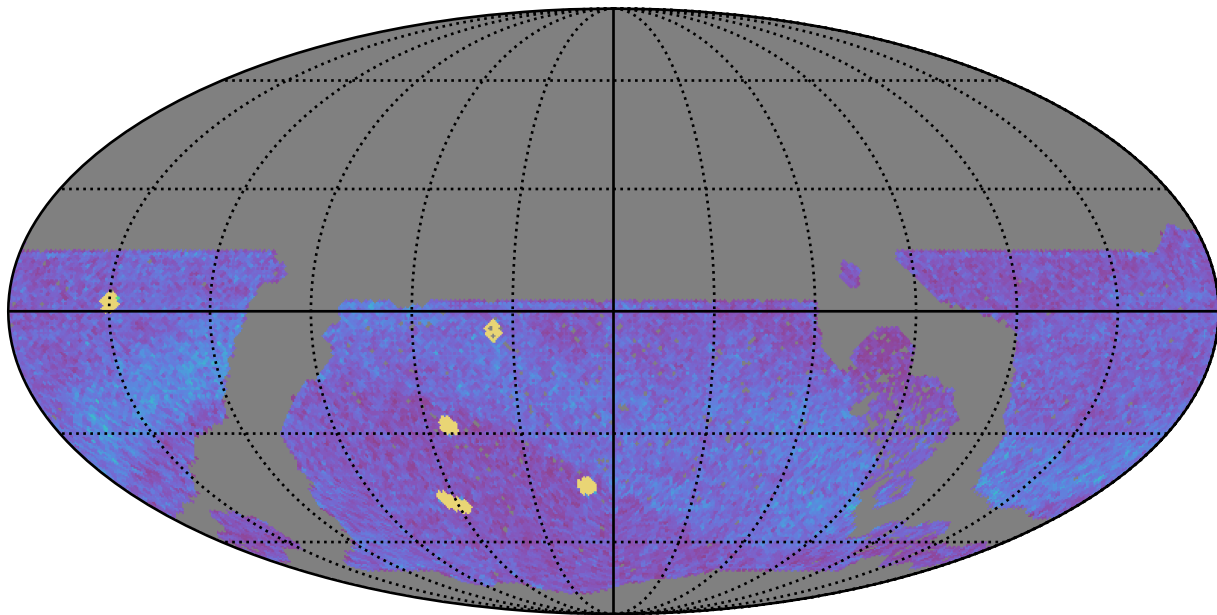
roll_pause_mjdp120_v3.4_10yrs WFD all bands: NVisits
