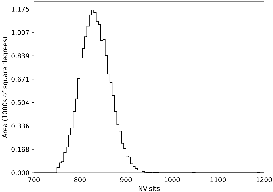
roll_pause_mjdp120_v3.4_10yrs WFD all bands: NVisits
