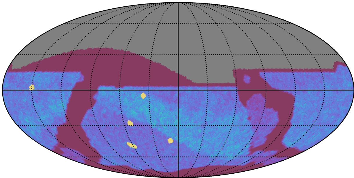
roll_pause_mjdp120_v3.4_10yrs All sky z band: NVisits
