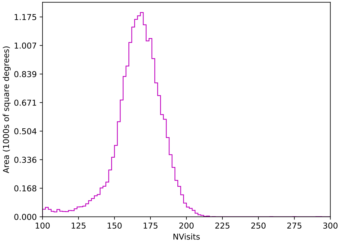
roll_pause_mjdp120_v3.4_10yrs All sky z band: NVisits
