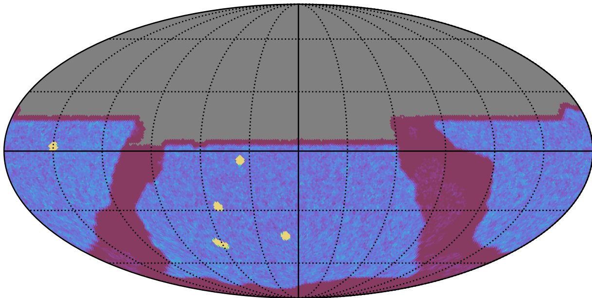
roll_pause_mjdp120_v3.4_10yrs All sky y band: NVisits
