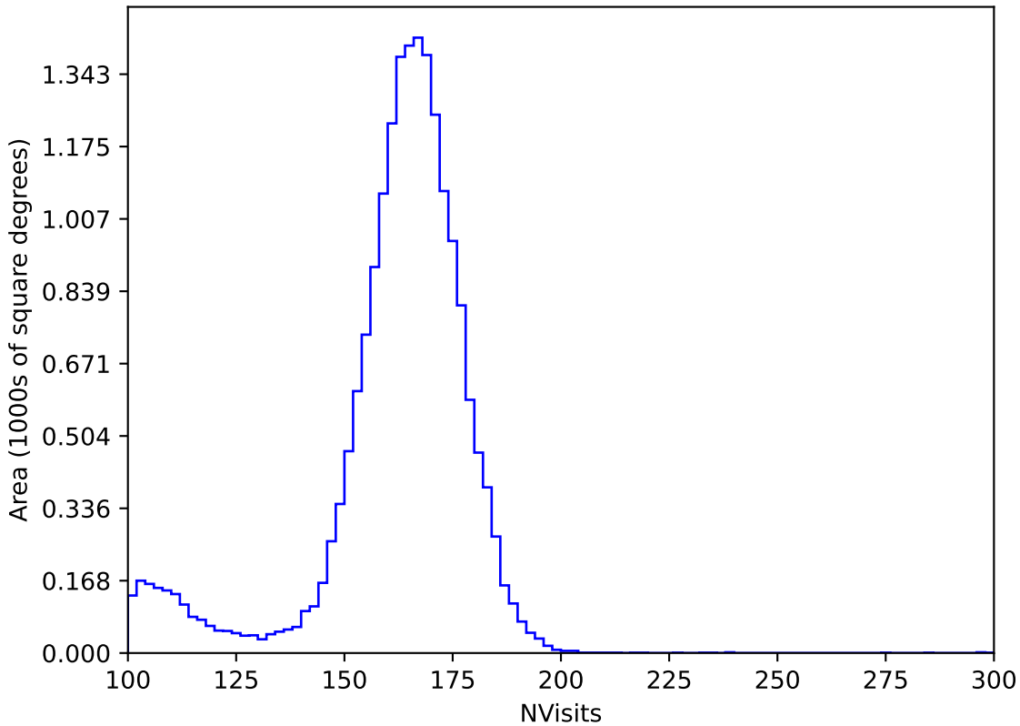
roll_pause_mjdp120_v3.4_10yrs All sky y band: NVisits
