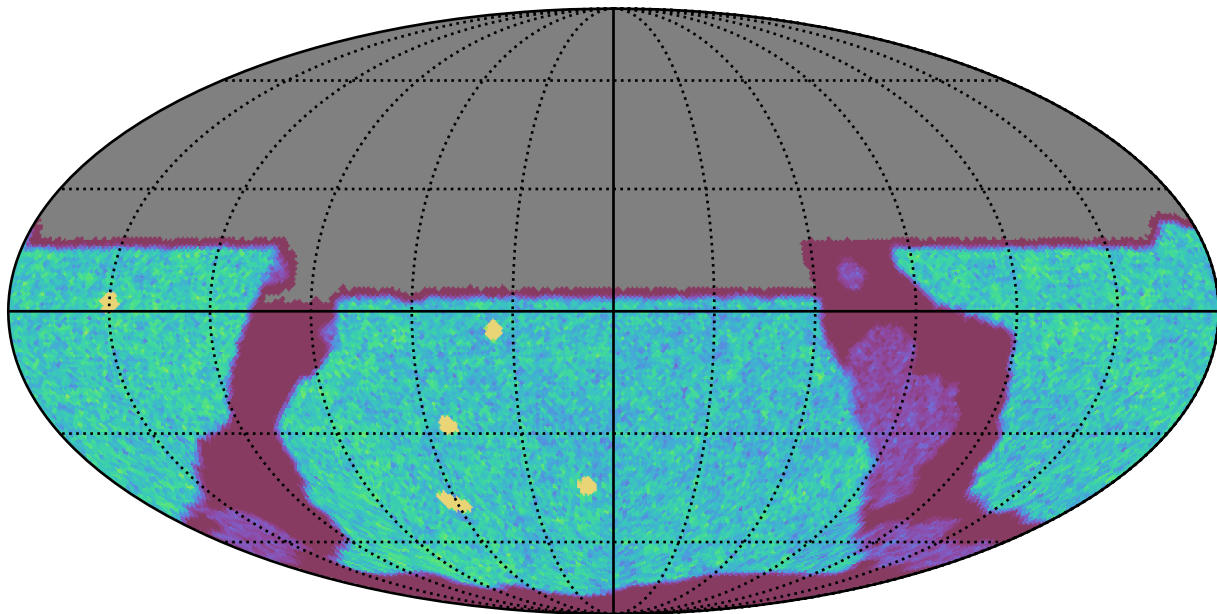
roll_pause_mjdp120_v3.4_10yrs All sky u band: NVisits
