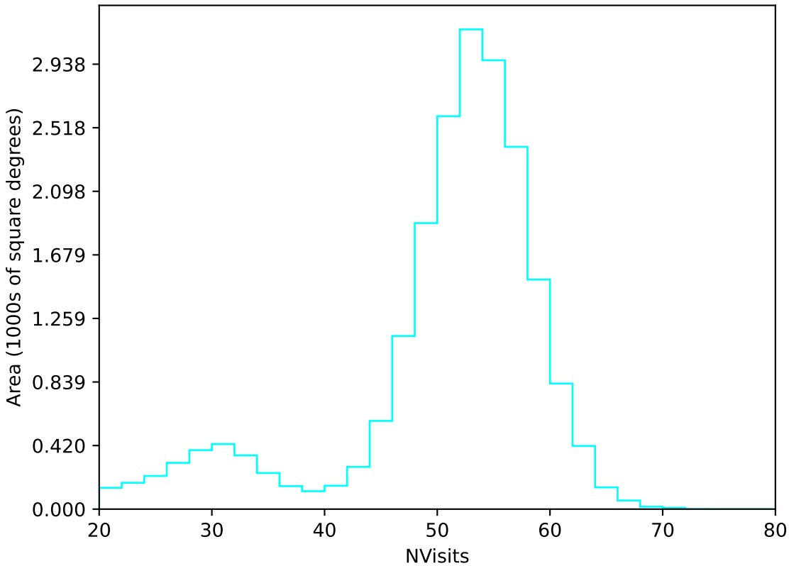
roll_pause_mjdp120_v3.4_10yrs All sky u band: NVisits
