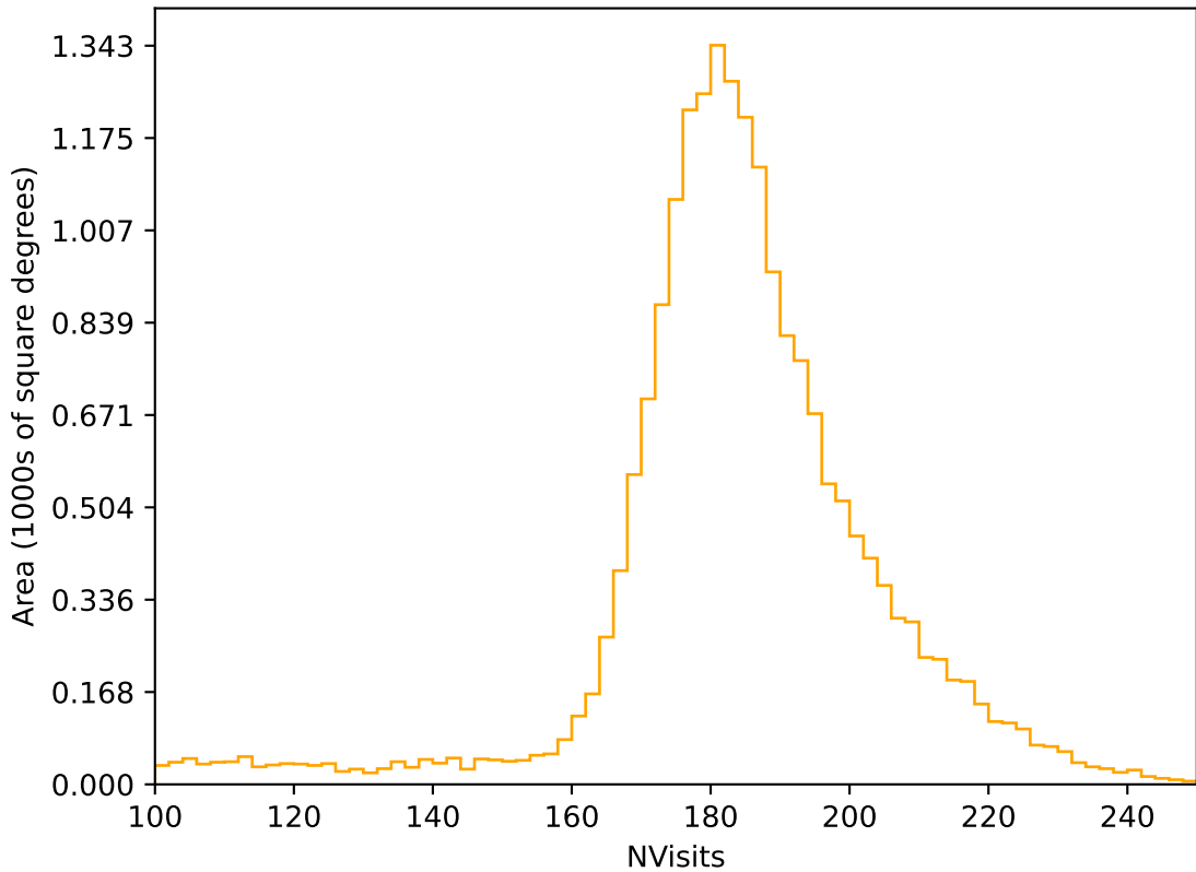
roll_pause_mjdp120_v3.4_10yrs All sky r band: NVisits
