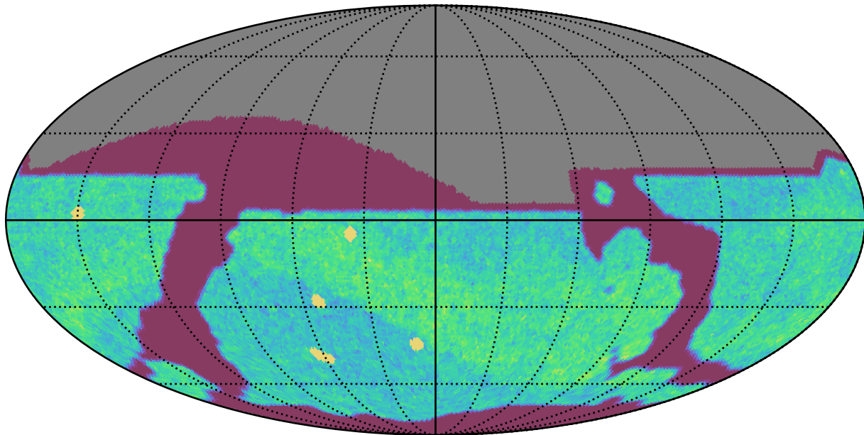
roll_pause_mjdp120_v3.4_10yrs All sky i band: NVisits
