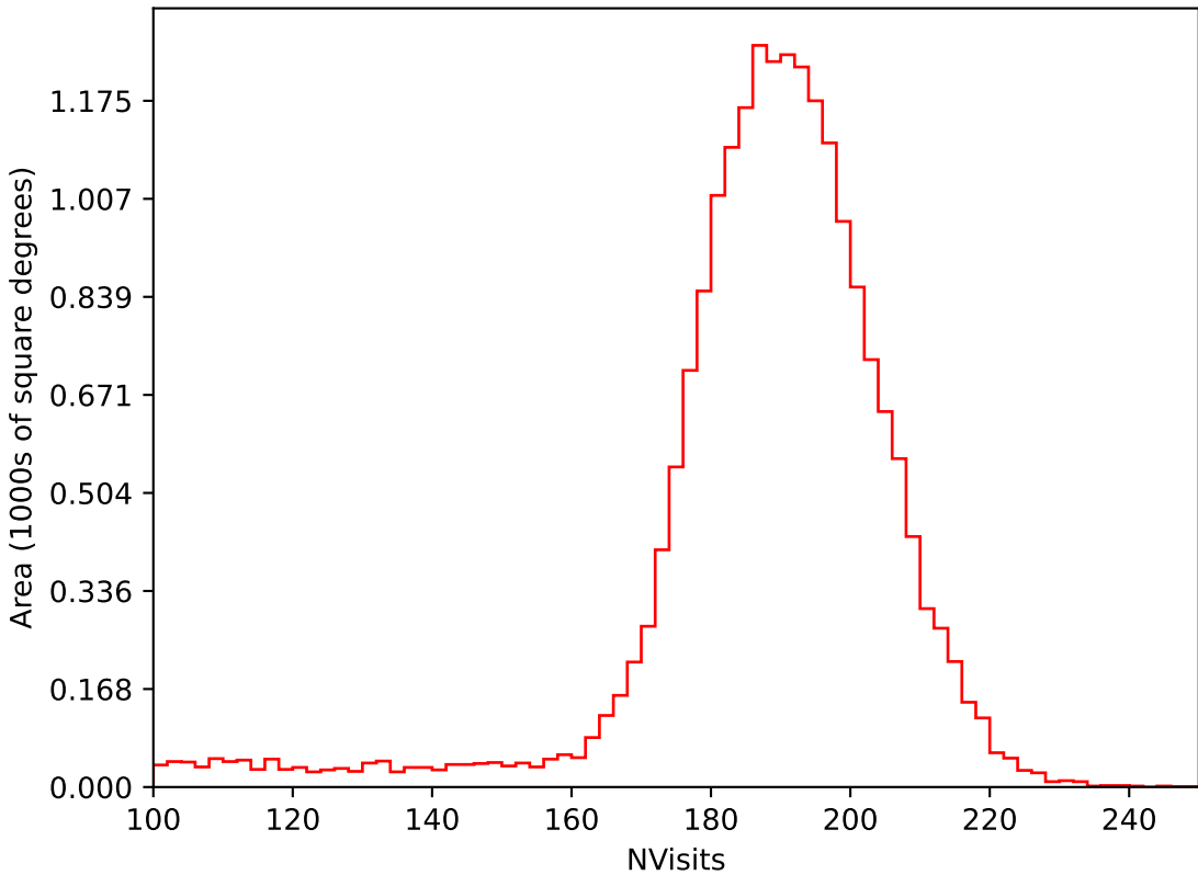
roll_pause_mjdp120_v3.4_10yrs All sky i band: NVisits
