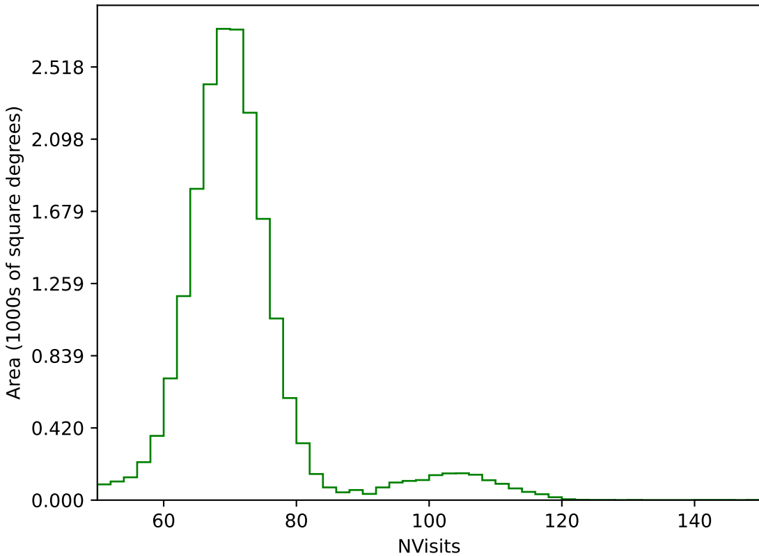
roll_pause_mjdp120_v3.4_10yrs All sky g band: NVisits
