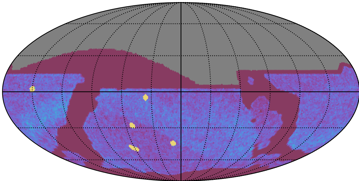
roll_pause_mjdp120_v3.4_10yrs All sky all bands: NVisits
