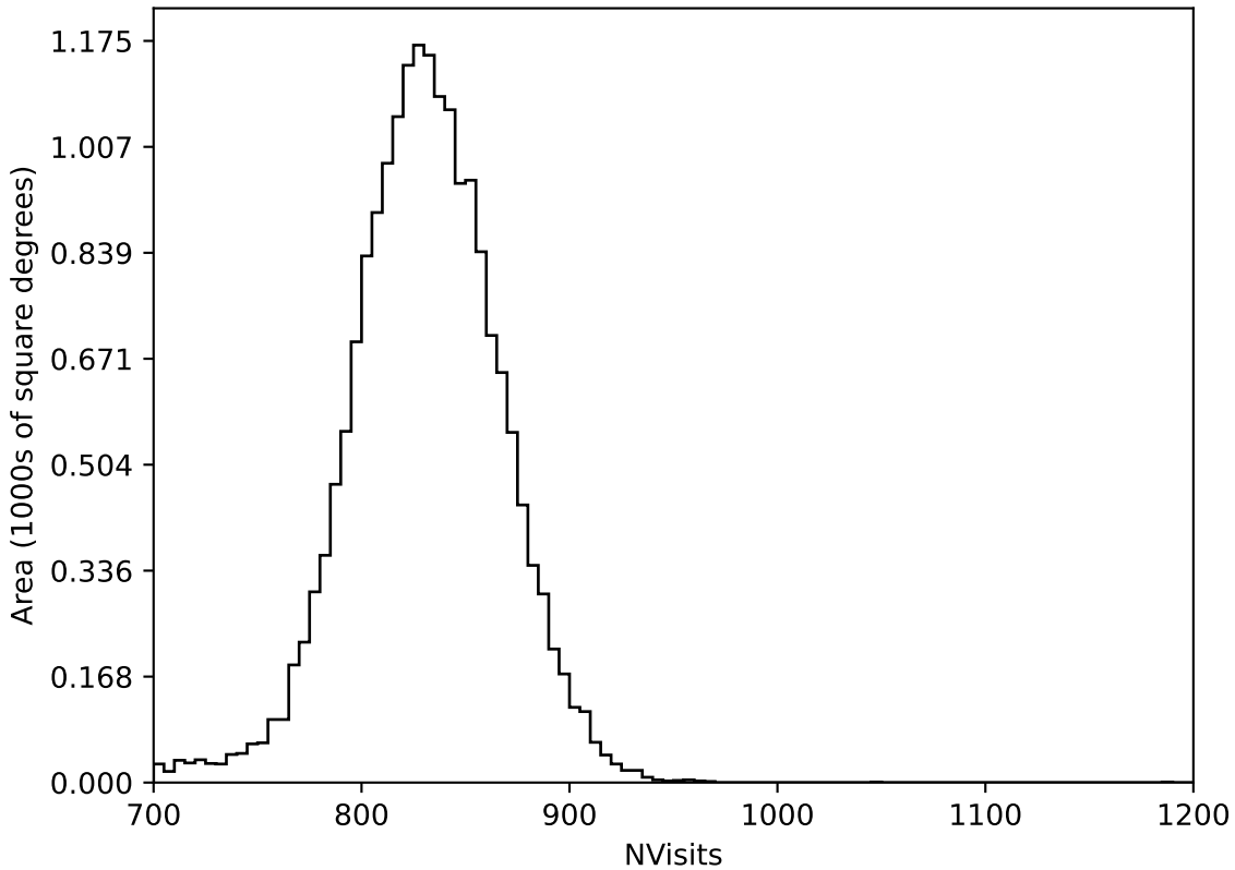
roll_pause_mjdp120_v3.4_10yrs All sky all bands: NVisits
