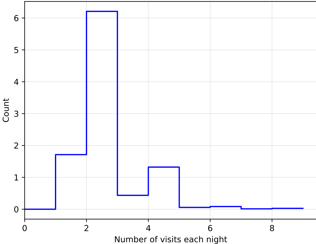
roll_pause_mjdp120_v3.4_10yrs All sky: NVisitsPerNight
