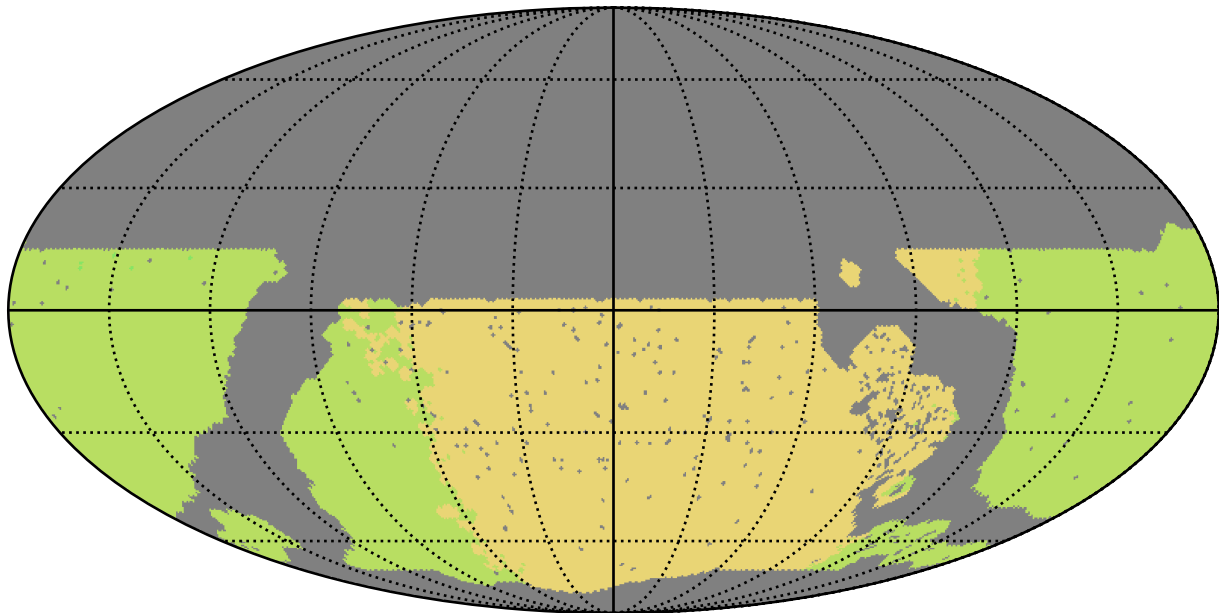
roll_pause_mjdp120_v3.4_10yrs WFD all bands: NSeasons
