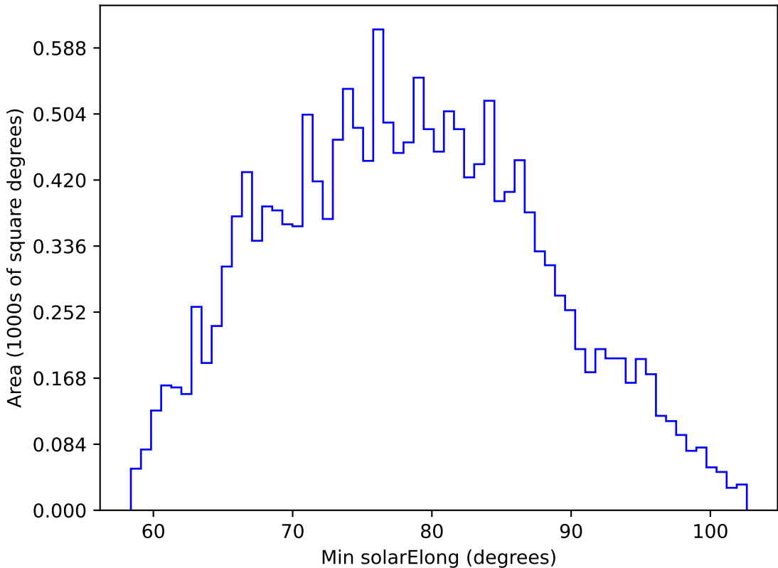
roll_pause_mjdp120_v3.4_10yrs WFD u band: Min solarElong
