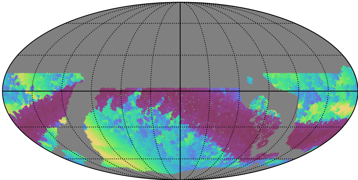
roll_pause_mjdp120_v3.4_10yrs WFD r band: Min solarElong
