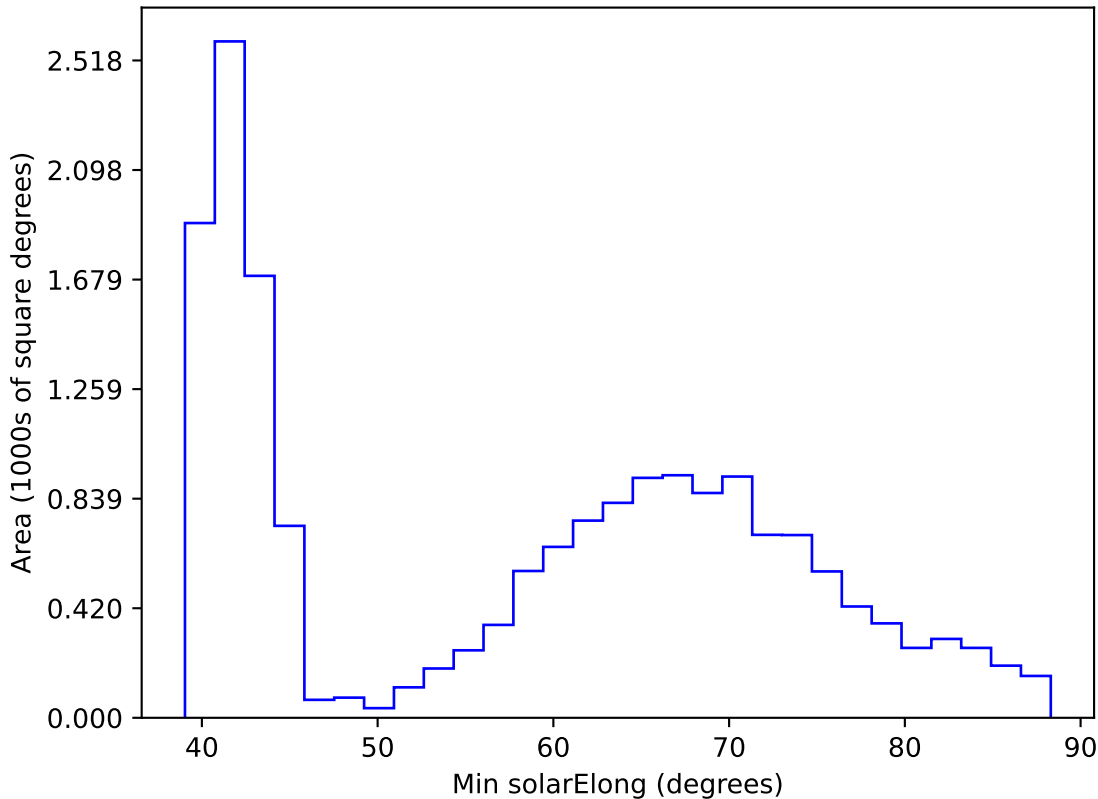
roll_pause_mjdp120_v3.4_10yrs WFD r band: Min solarElong
