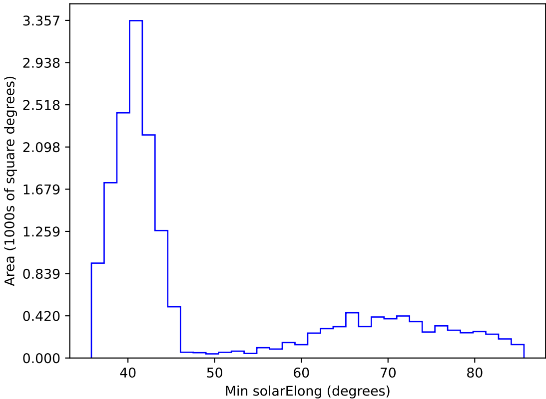
roll_pause_mjdp120_v3.4_10yrs WFD i band: Min solarElong
