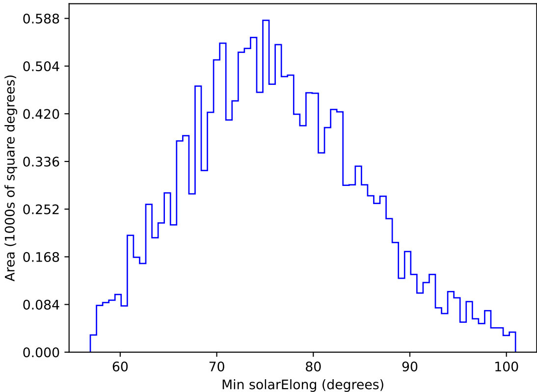
roll_pause_mjdp120_v3.4_10yrs WFD g band: Min solarElong
