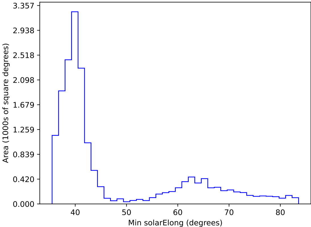
roll_pause_mjdp120_v3.4_10yrs WFD all bands: Min solarElong
