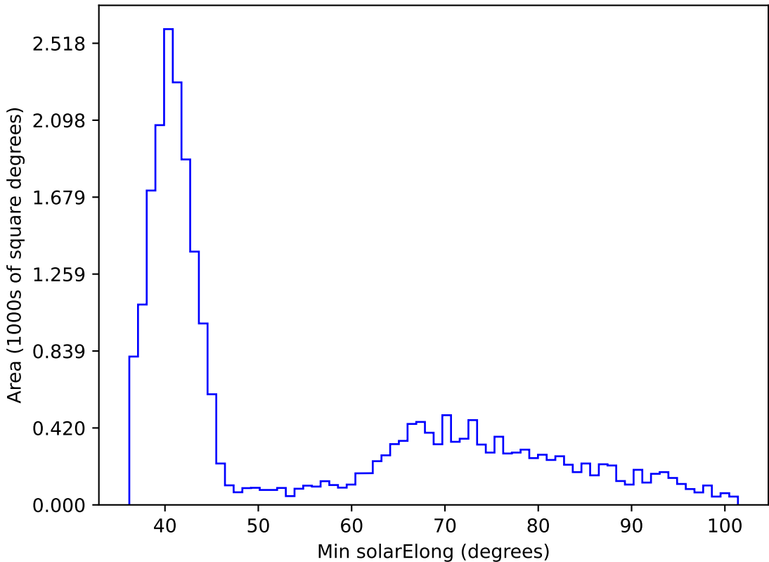
roll_pause_mjdp120_v3.4_10yrs All sky z band: Min solarElong
