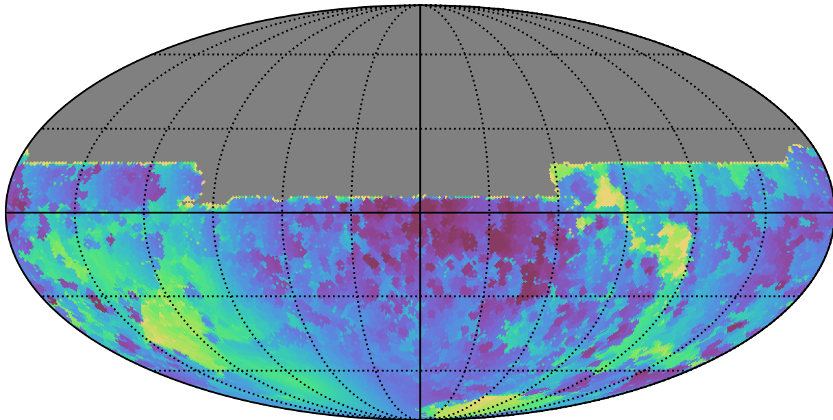
roll_pause_mjdp120_v3.4_10yrs All sky y band: Min solarElong
