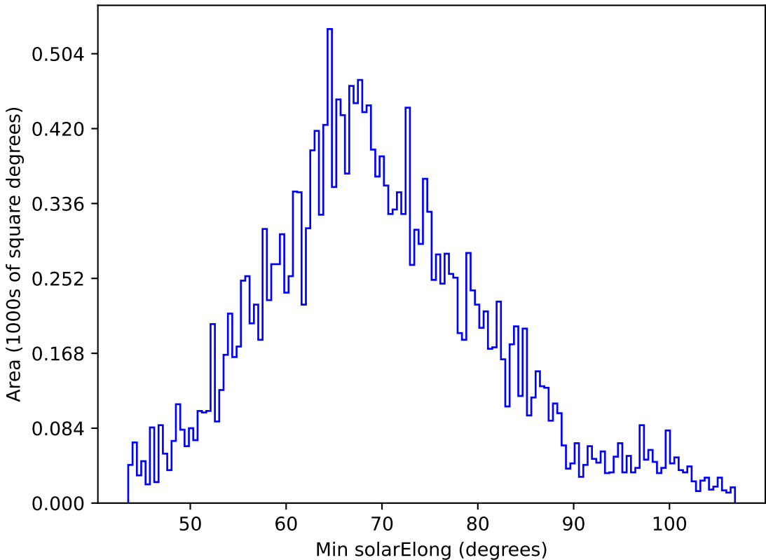
roll_pause_mjdp120_v3.4_10yrs All sky y band: Min solarElong
