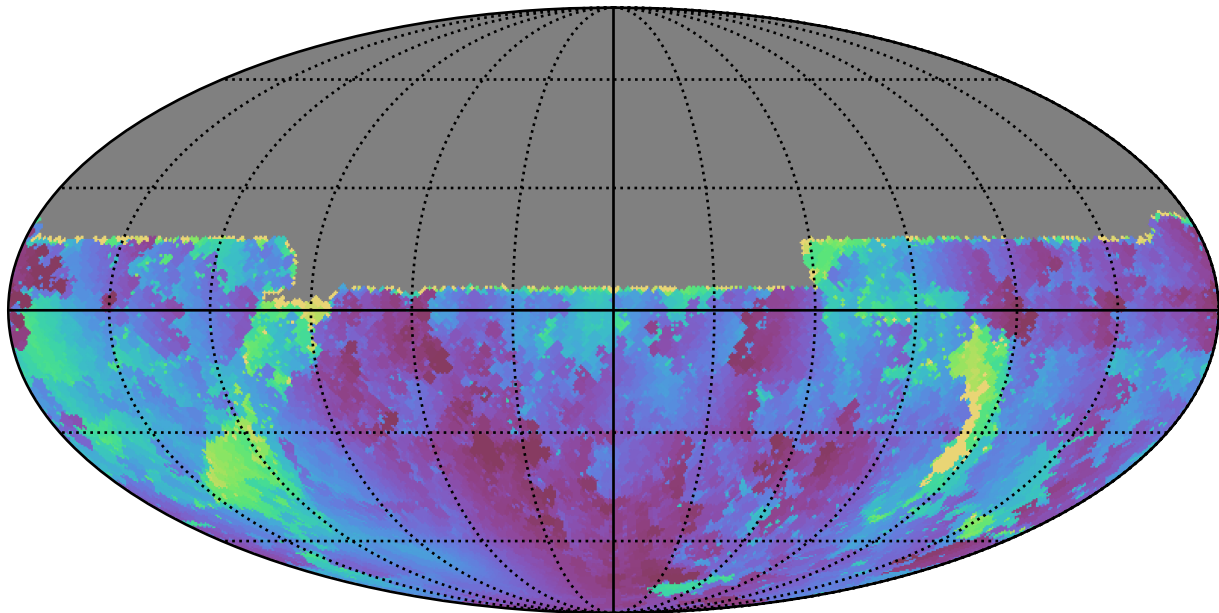
roll_pause_mjdp120_v3.4_10yrs All sky u band: Min solarElong
