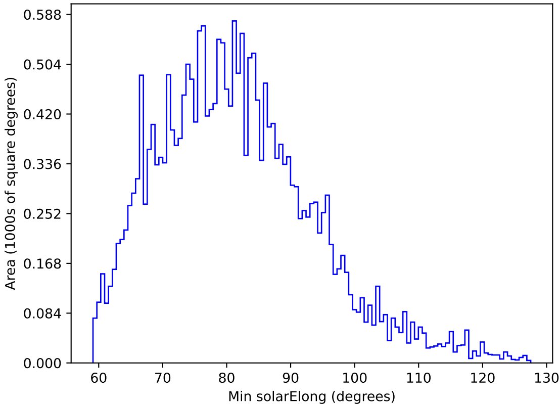
roll_pause_mjdp120_v3.4_10yrs All sky u band: Min solarElong
