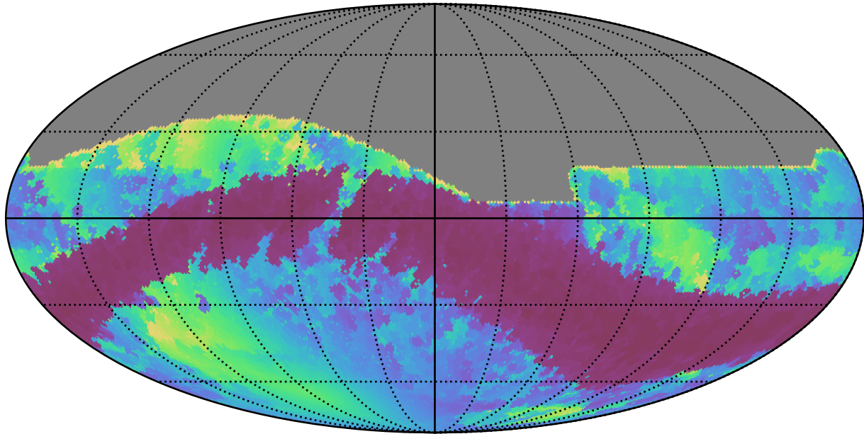
roll_pause_mjdp120_v3.4_10yrs All sky r band: Min solarElong
