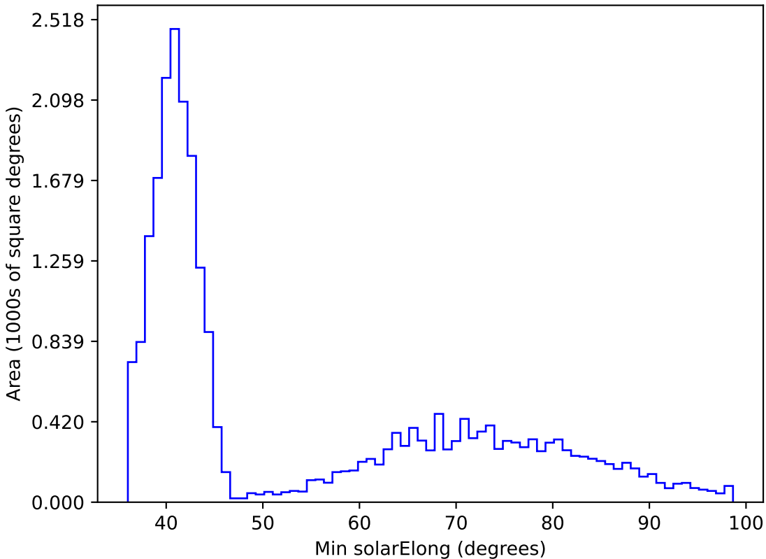
roll_pause_mjdp120_v3.4_10yrs All sky i band: Min solarElong
