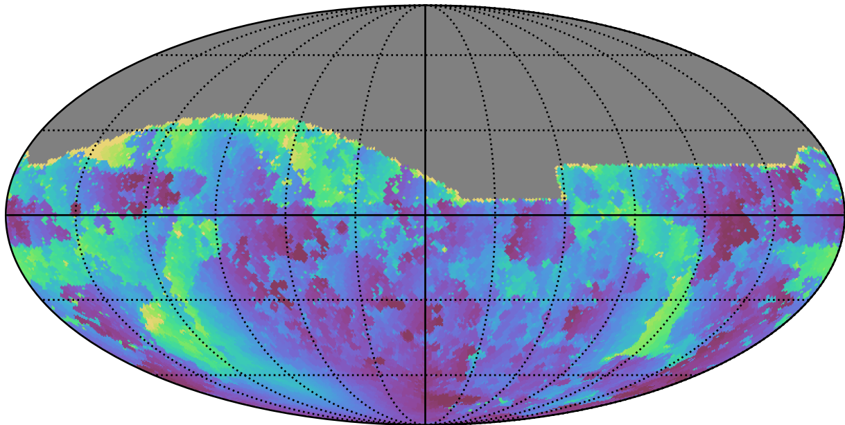
roll_pause_mjdp120_v3.4_10yrs All sky g band: Min solarElong
