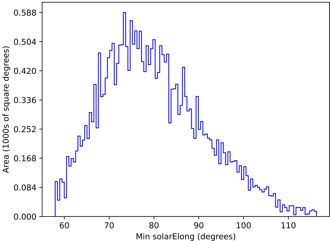
roll_pause_mjdp120_v3.4_10yrs All sky g band: Min solarElong
