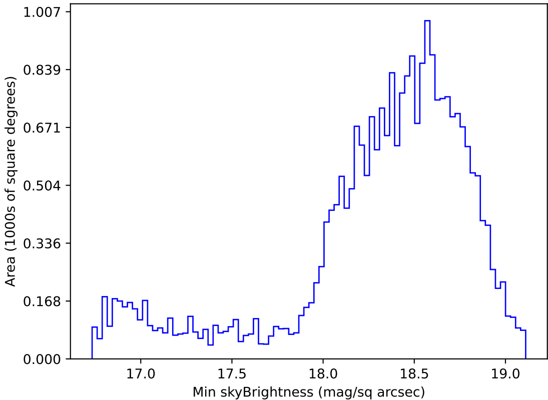
roll_pause_mjdp120_v3.4_10yrs Yr 1 z band: Min skyBrightness
