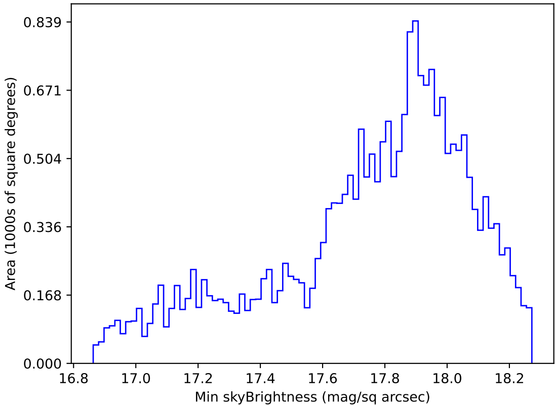
roll_pause_mjdp120_v3.4_10yrs Yr 1 y band: Min skyBrightness
