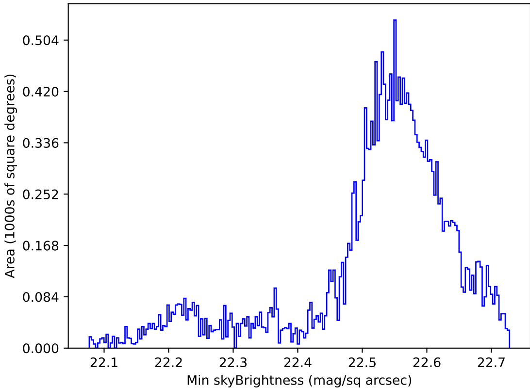
roll_pause_mjdp120_v3.4_10yrs Yr 1 u band: Min skyBrightness
