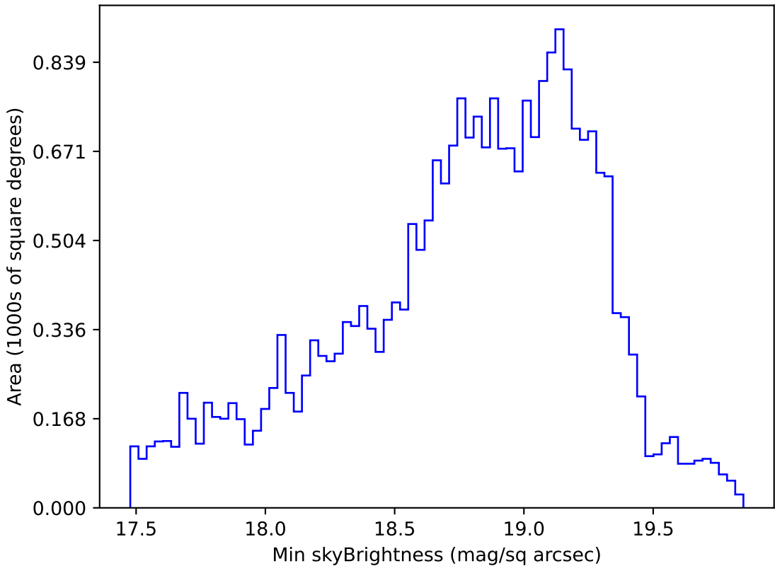
roll_pause_mjdp120_v3.4_10yrs Yr 1 i band: Min skyBrightness
