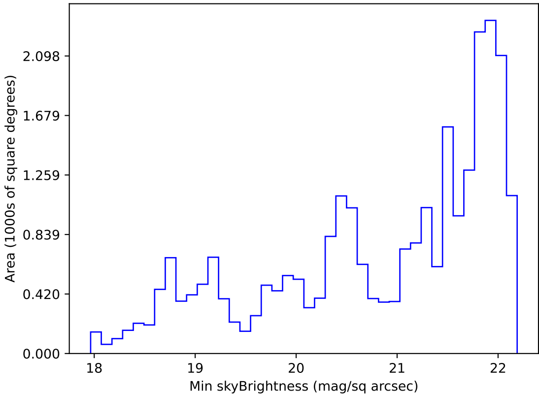
roll_pause_mjdp120_v3.4_10yrs Yr 1 g band: Min skyBrightness
