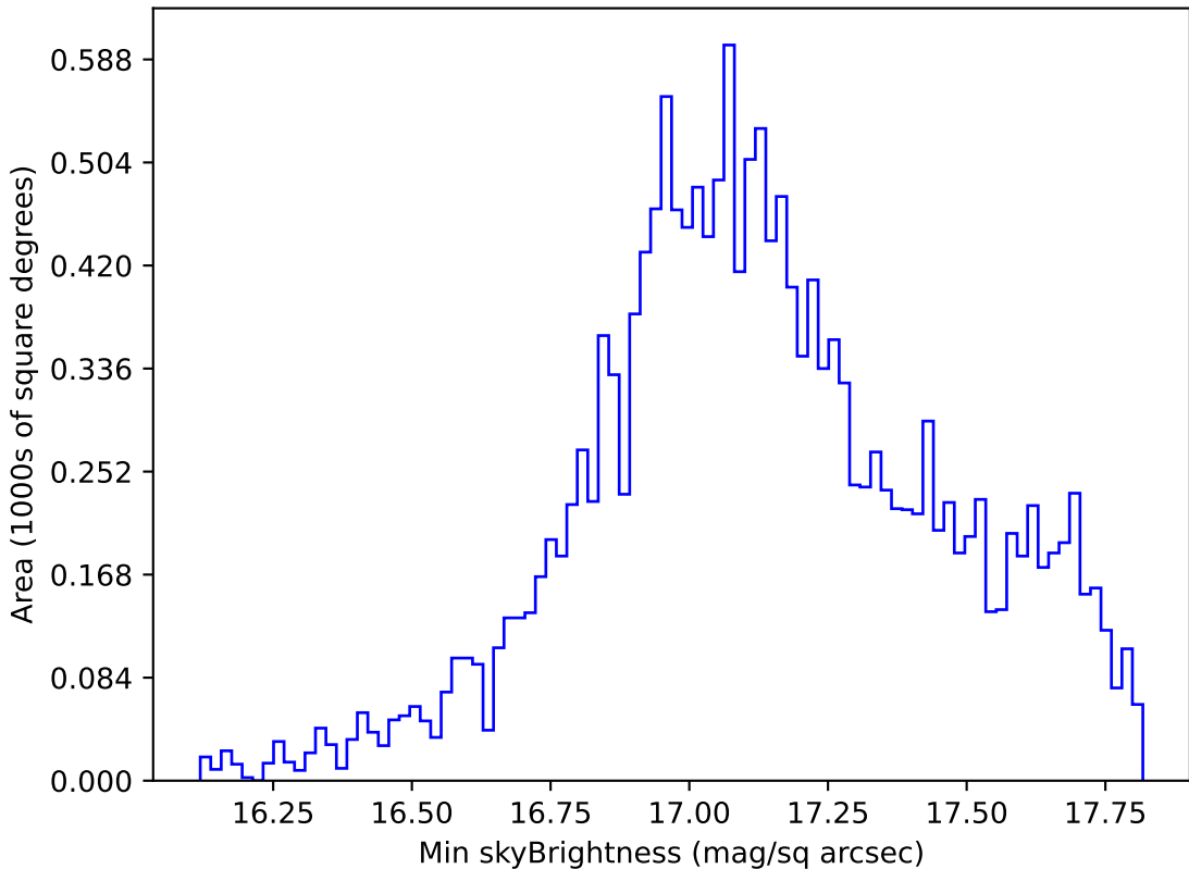
roll_pause_mjdp120_v3.4_10yrs WFD y band: Min skyBrightness
