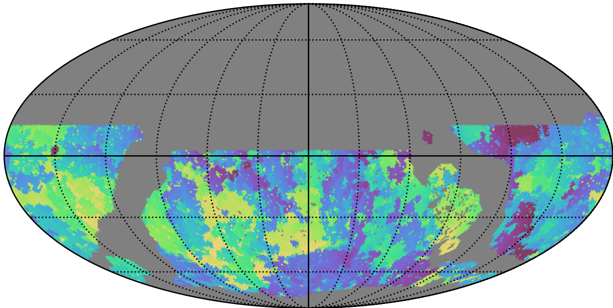
roll_pause_mjdp120_v3.4_10yrs WFD u band: Min skyBrightness
