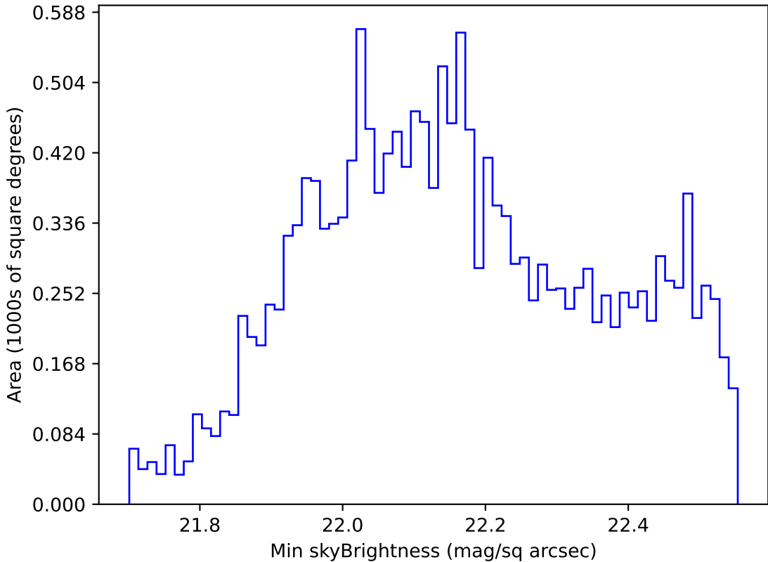
roll_pause_mjdp120_v3.4_10yrs WFD u band: Min skyBrightness
