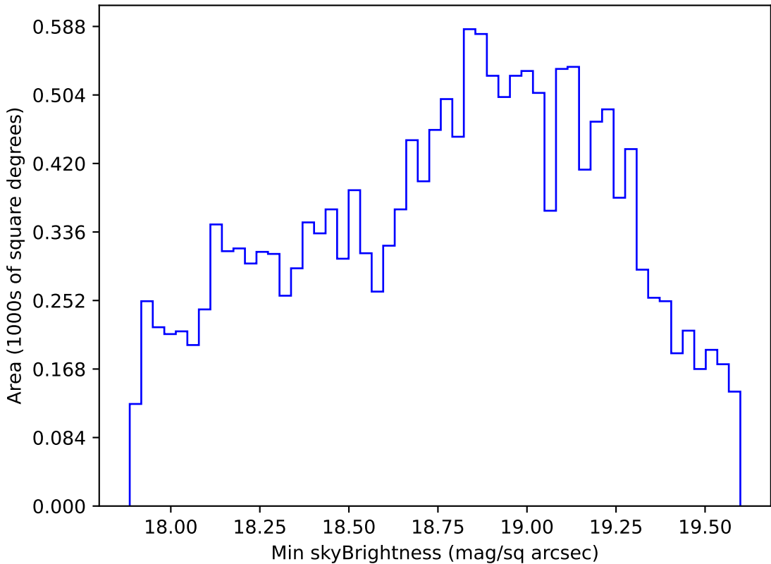
roll_pause_mjdp120_v3.4_10yrs WFD r band: Min skyBrightness
