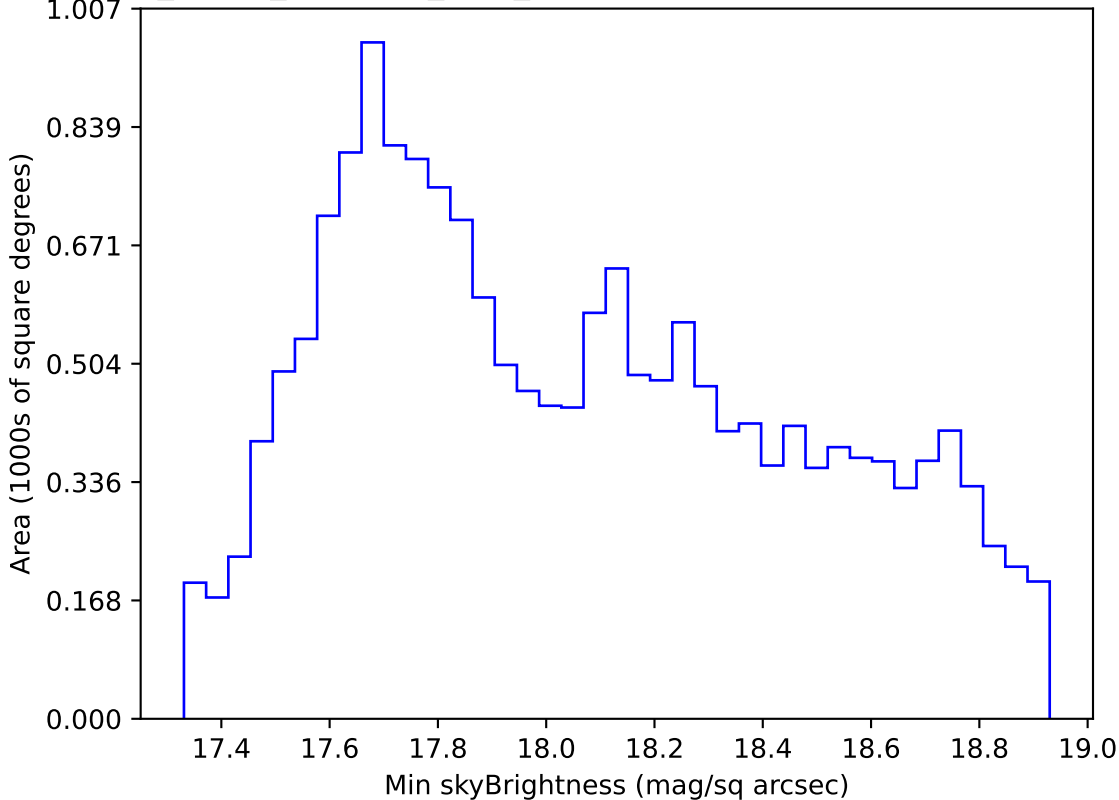
roll_pause_mjdp120_v3.4_10yrs WFD i band: Min skyBrightness
