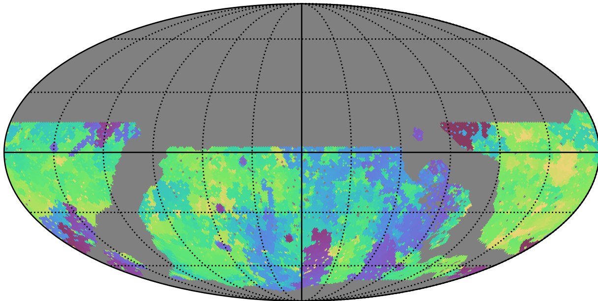
roll_pause_mjdp120_v3.4_10yrs WFD g band: Min skyBrightness
