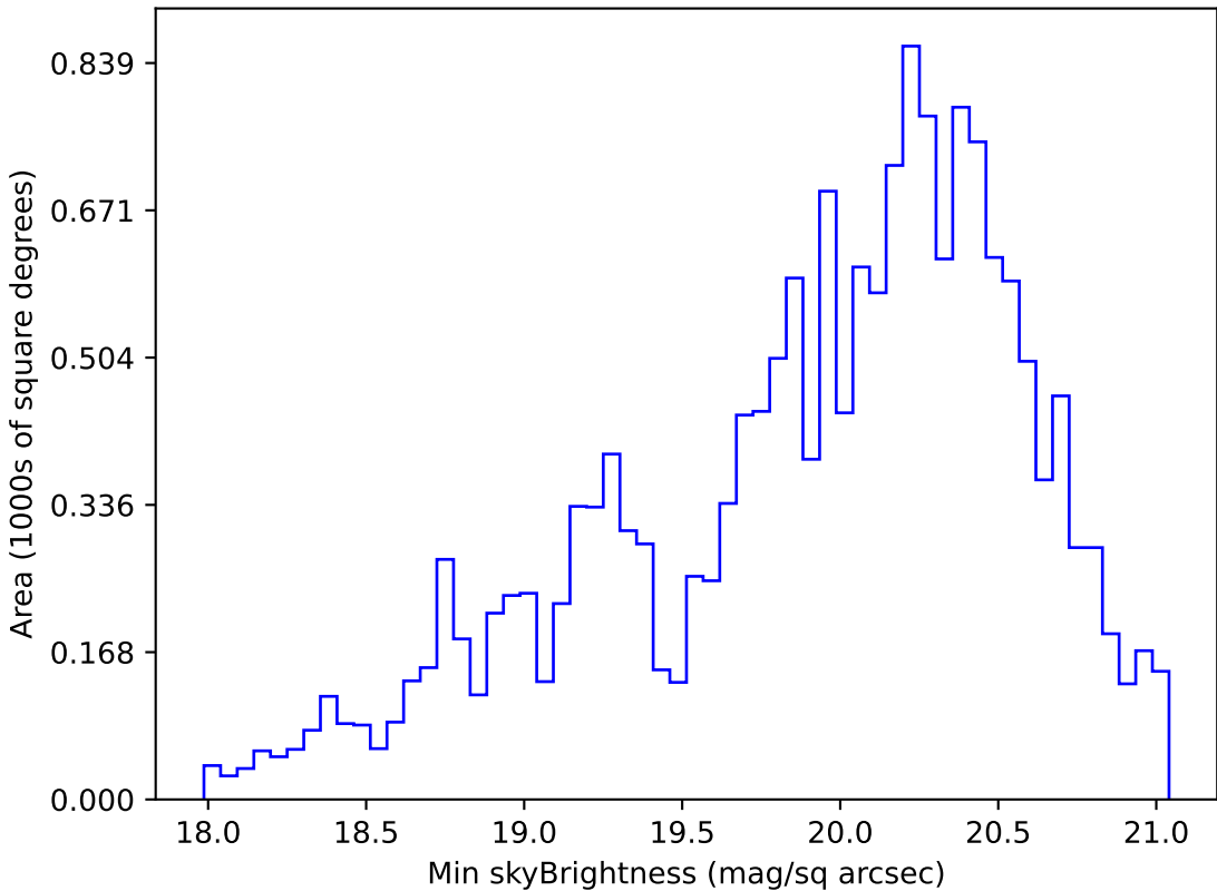
roll_pause_mjdp120_v3.4_10yrs WFD g band: Min skyBrightness
