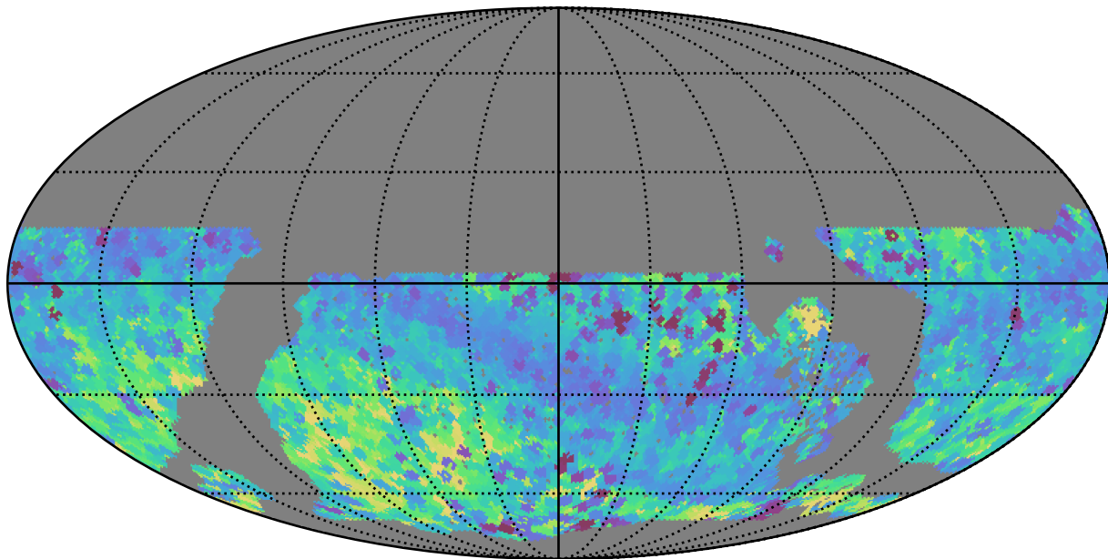
roll_pause_mjdp120_v3.4_10yrs WFD all bands: Min skyBrightness
