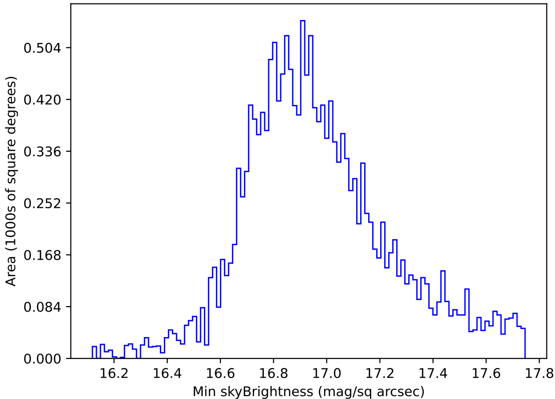
roll_pause_mjdp120_v3.4_10yrs WFD all bands: Min skyBrightness
